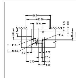
RJX8FD*HB (Front Mounting)
