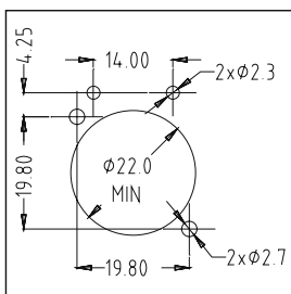
PANEL CUTOUP A and B type with LED's
